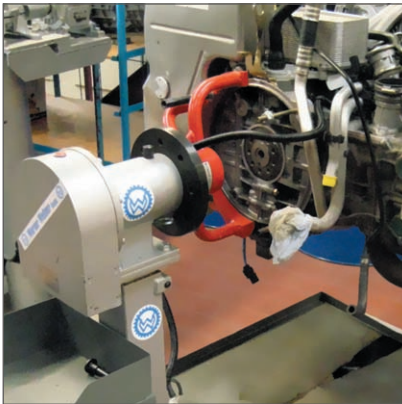
Application with porsche adaptor
