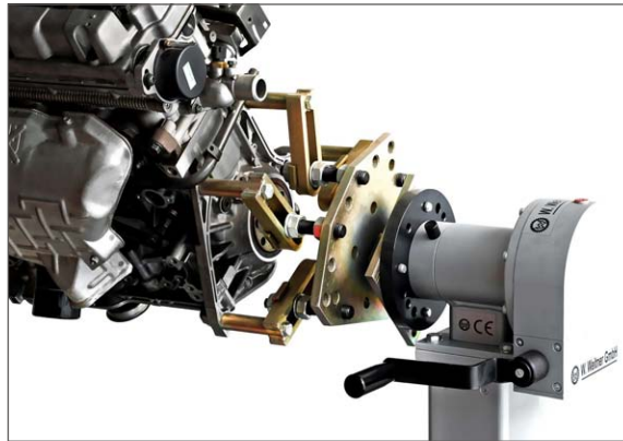
Application with ww-4/100 Universal support
