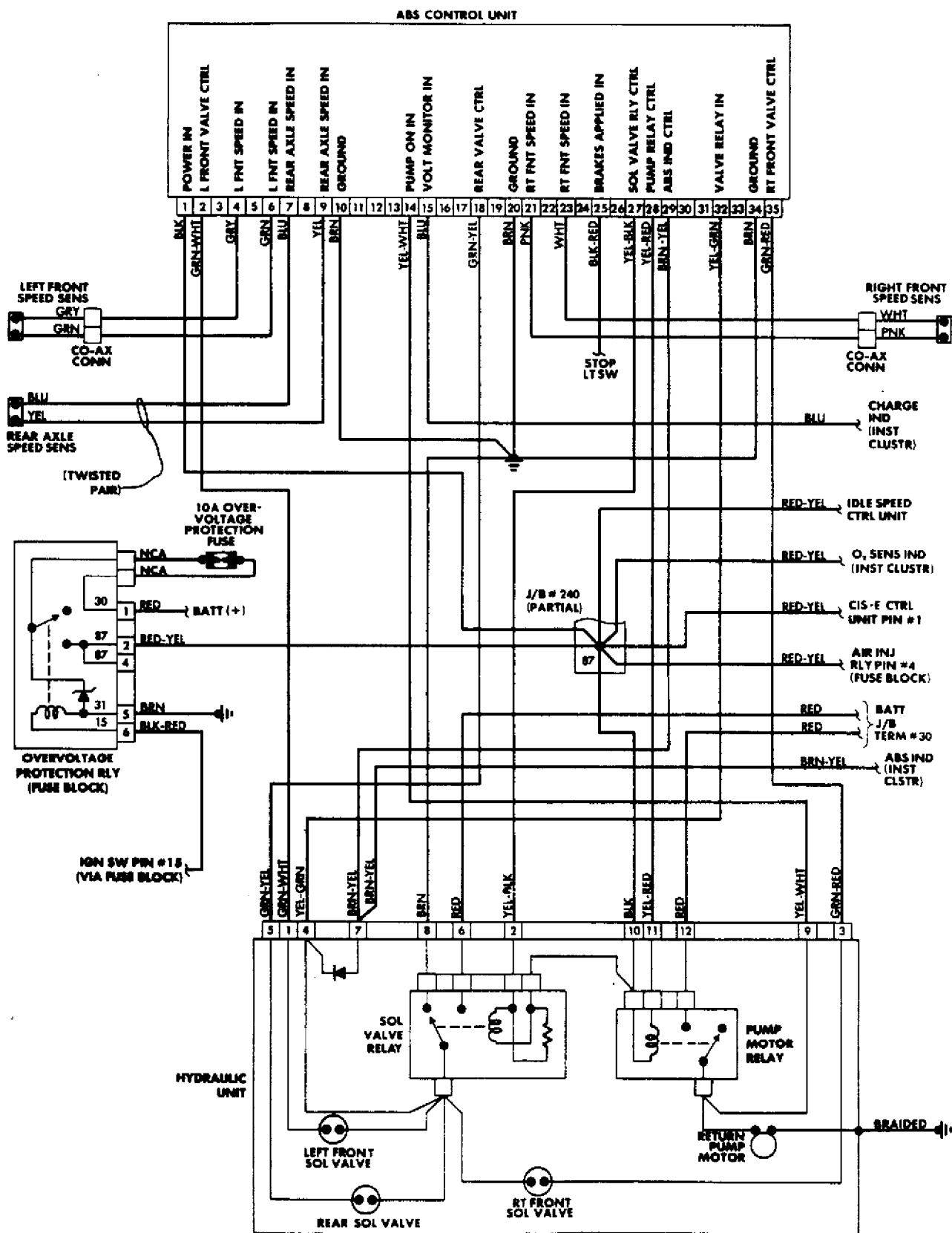
Fig. 7: Mercedes-Benz 560 Series Anti-Lock Brake System Wiring Diagram
