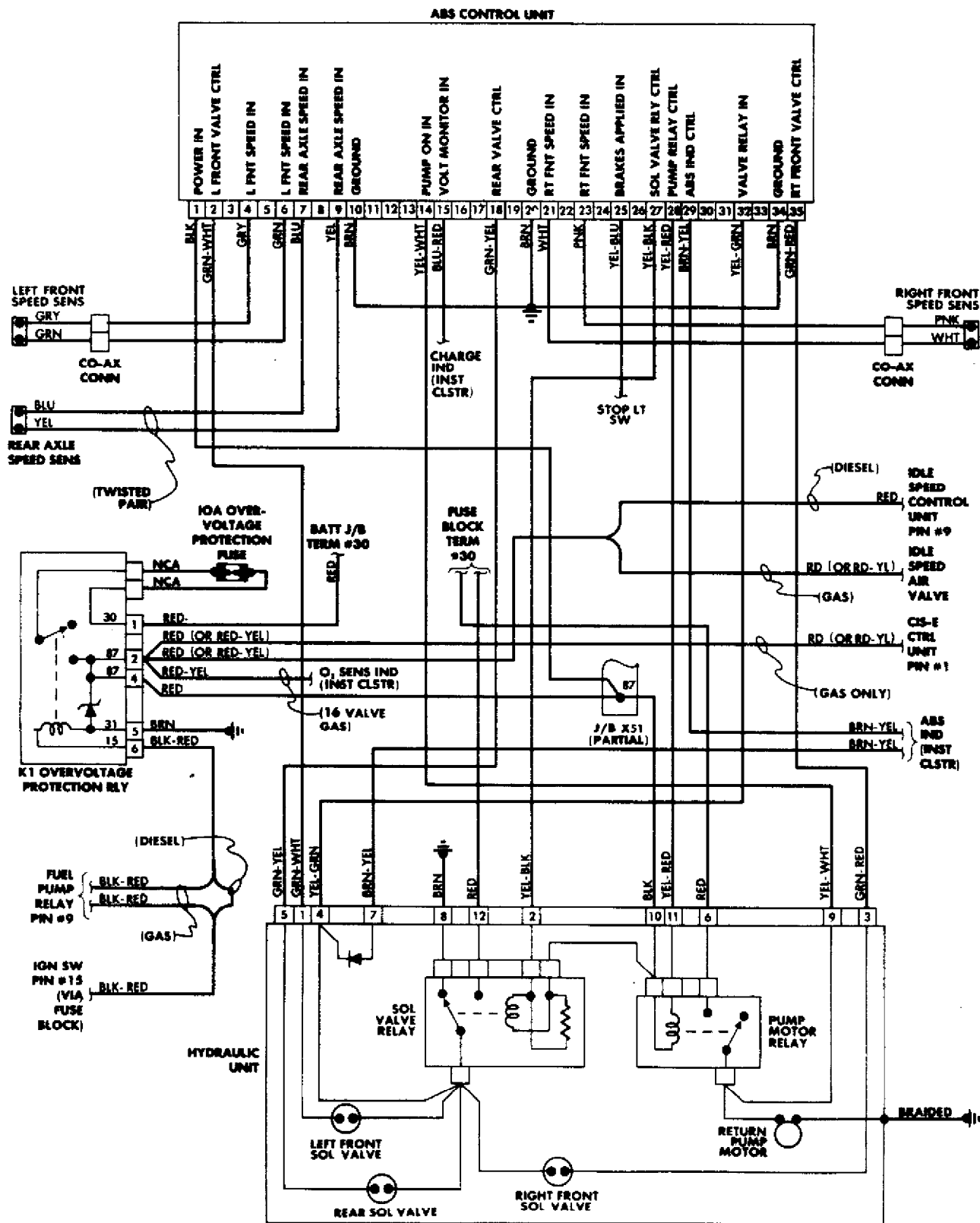
Fig. 4: Mercedes-Benz 190E Anti-Lock Brake System Wiring Diagram
