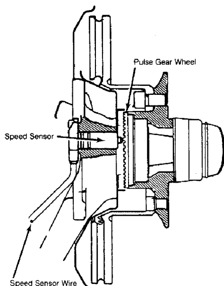
Fig. 2: Cutaway View Of Mercedes-Benz ABS Front Speed Sensor Assembly Courtesy of Mercedes-Benz of North America.
