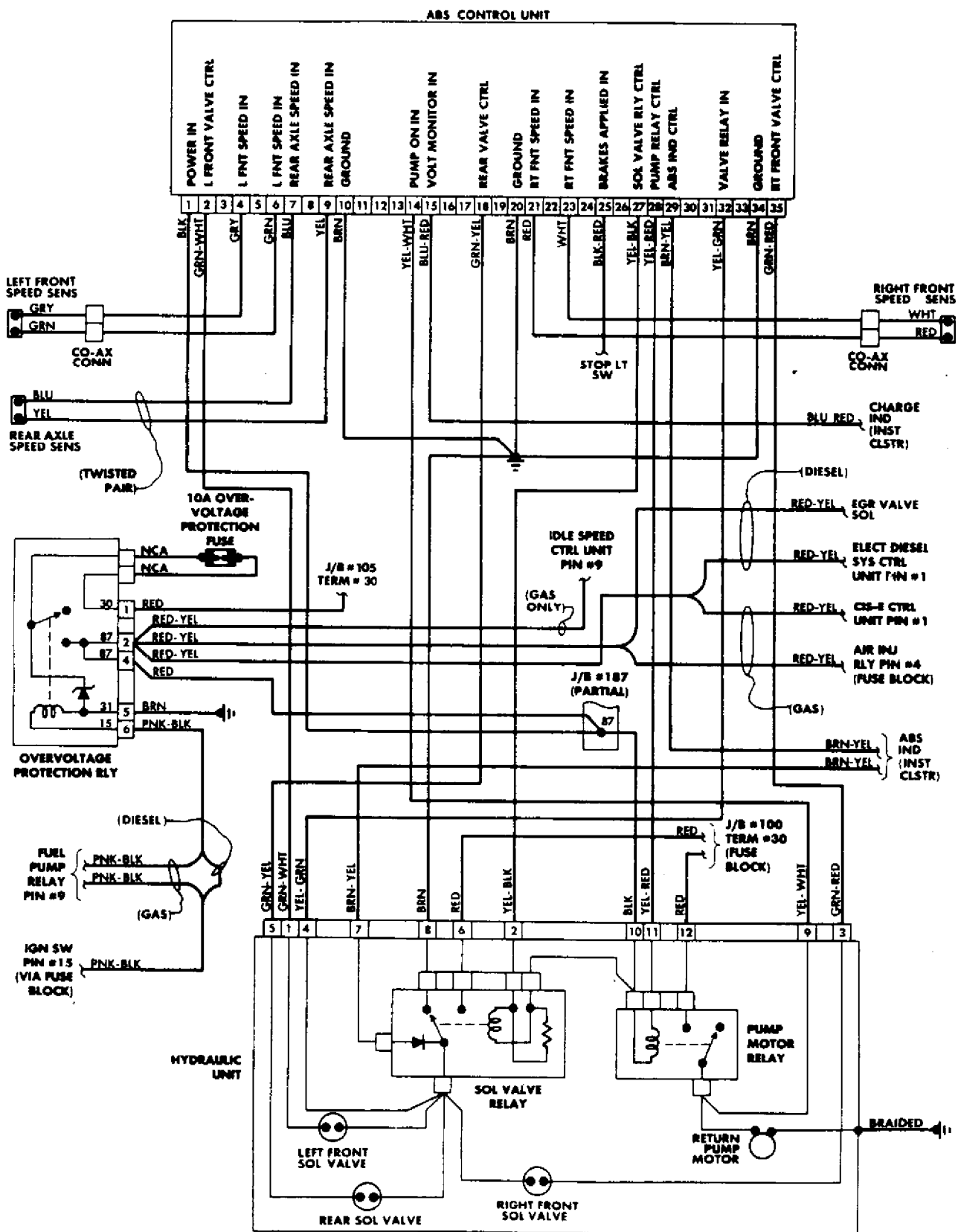
Fig. 6: Mercedes-Benz 420SEL Anti-Lock Brake System Wiring Diagram
