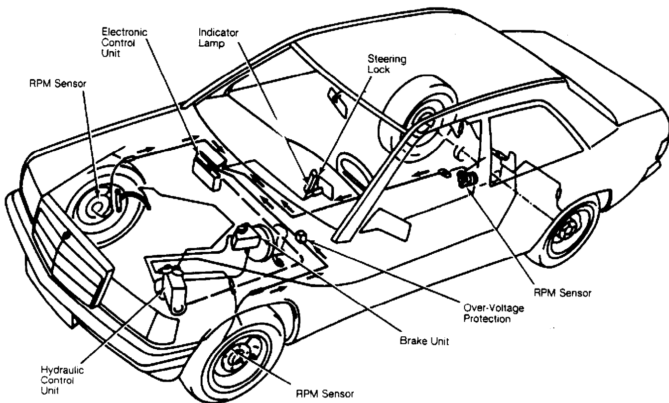
Fig. 1: Mercedes-Benz ABS Component Location Courtesy of Mercedes-Benz of North America.
