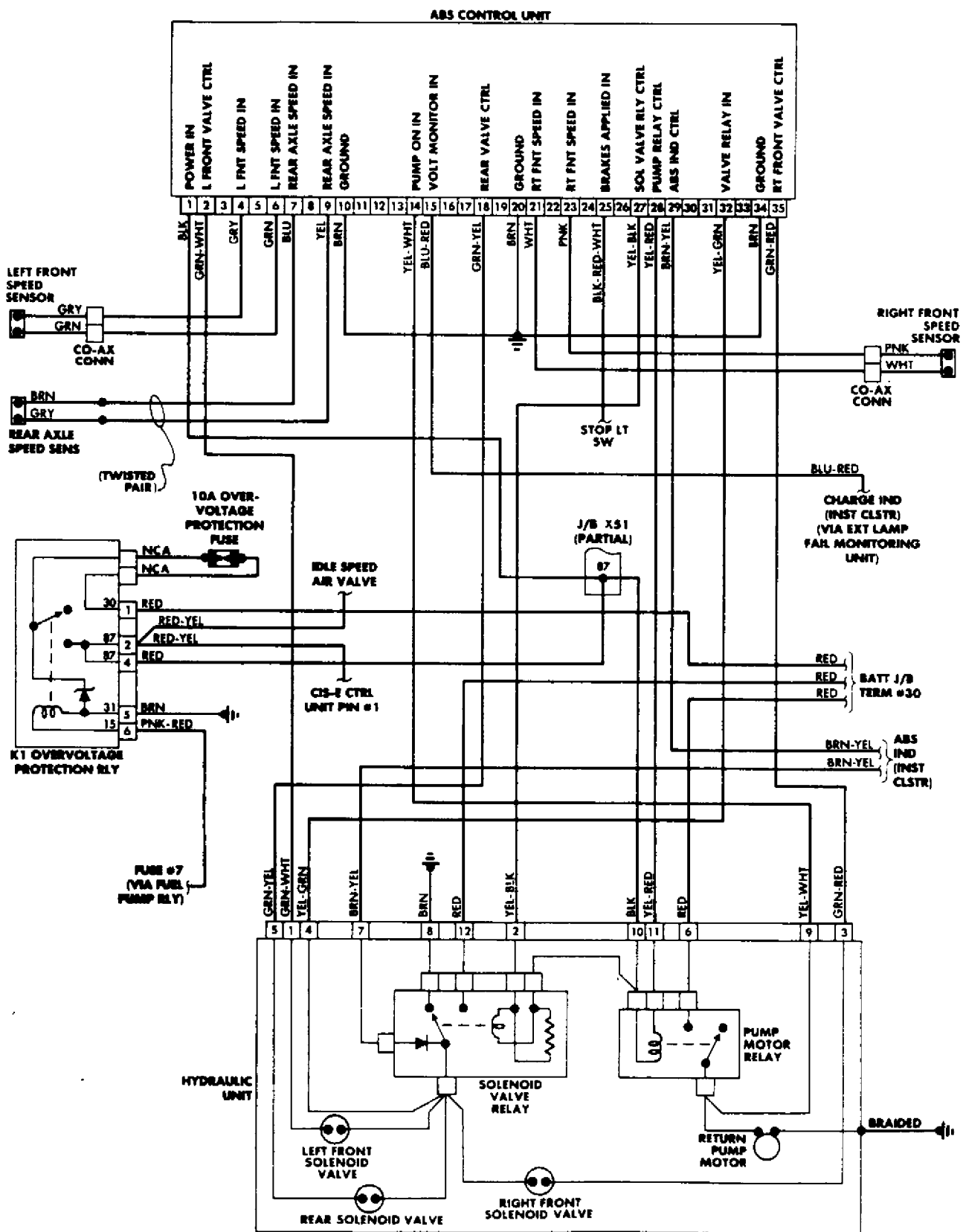
Fig. 5: Mercedes-Benz 260E & 300 Series Anti-Lock Brake System Wiring Diagram
